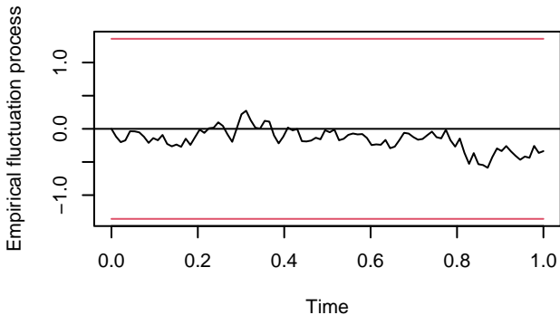
OLS-CUSUM of equation Oil.Gas.Ratio
